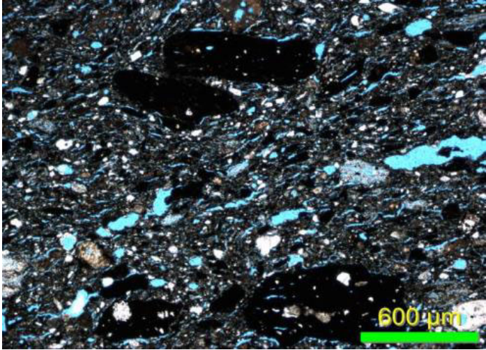
Figure 30. Yingjing soup pot thin section in plane polarized light is filled with fine-grained quartz, large fragments of coal, and smaller coal ash particles.
