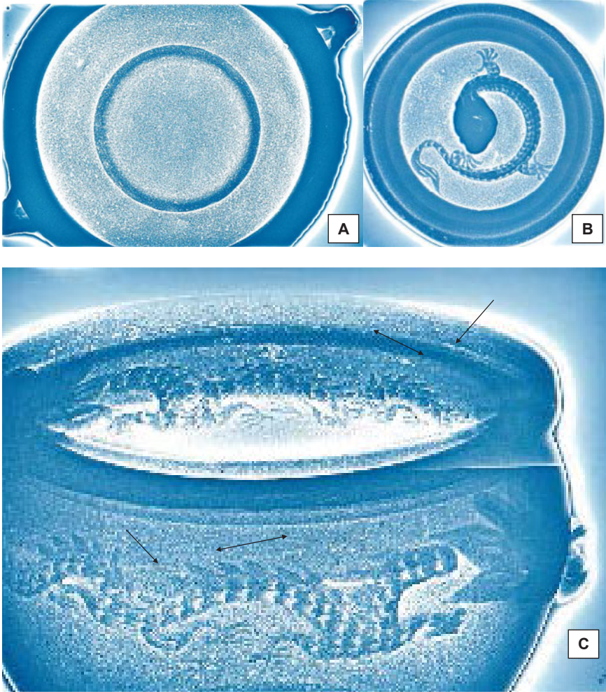
Figure 14. The Yijing soup pot has a molded base and lower wall with randomly oriented porosity (A and C) and an upper wall with horizontal coil joints above the dragon and at the flange for the lid (single-pointed black arrows). These coils (C) were thrown on a fast wheel, shown by the diagonal alignment of porosity, as indicated by the double-ended black arrows set above the white-appearing lines of porosity. The lid (B) is decorated with a lucky dragon and has an even coarse texture with diagonal elongation of larger pores and strings of pores that indicates throwing. The two flanges of the lid are also visible.
