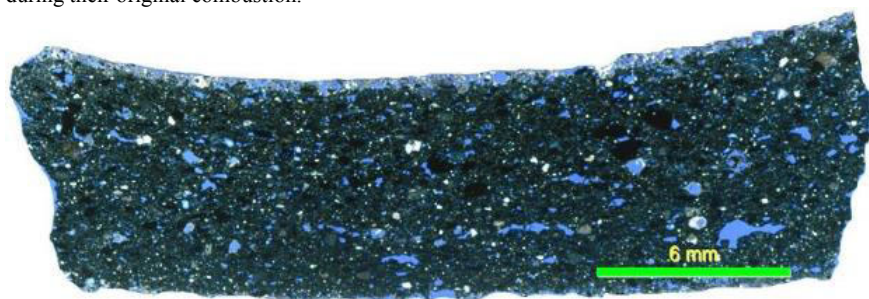
Figure 29. Yijing fired soup pot thin section, scanned at 2.5 \mu\text{m}/\text{pixel} , shows 12% Total Optical Porosity (TOP) with pores in a variety of sizes and shapes. Extremely fine porosity is present in the ash-glaze layer on the upper surface of the sherd.
