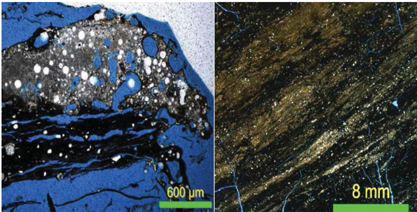
Figure 5. Yingjing “unqualified” glassy coal cinders with carbonized material below and mixed glass, pores, and crystalline phases above (left); and more homogeneous, low-glass phase “qualified” coal cinders (right).
