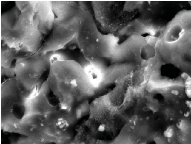
Figure 17. Enlargement of Fig. 16, showing well developed sintered microstructures of fired Yingjing soup pot at 8000x, with smooth surfaces on well-rounded pores and presence of fine rounded precipitates at glass-pore interfaces, perhaps mullite or an iron silicate.
